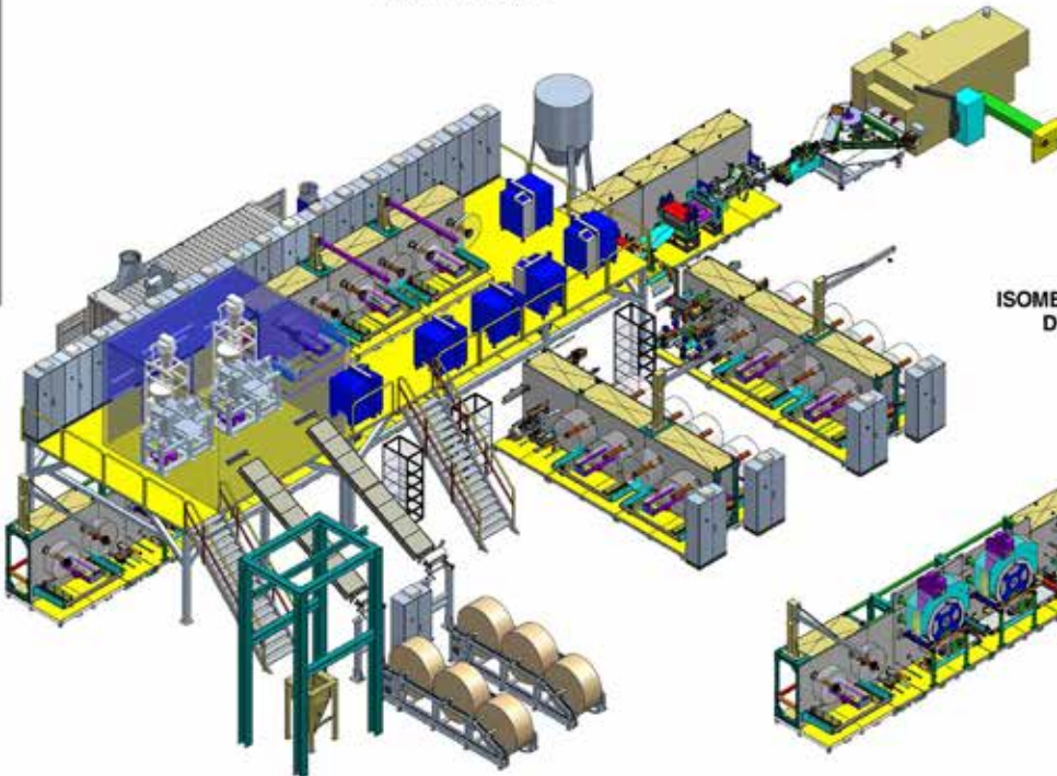
ISOMETRIC VIEW
