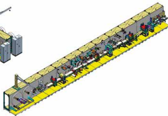
ISOMETRIC VIEW BOTTOM DETAIL MACHINE
