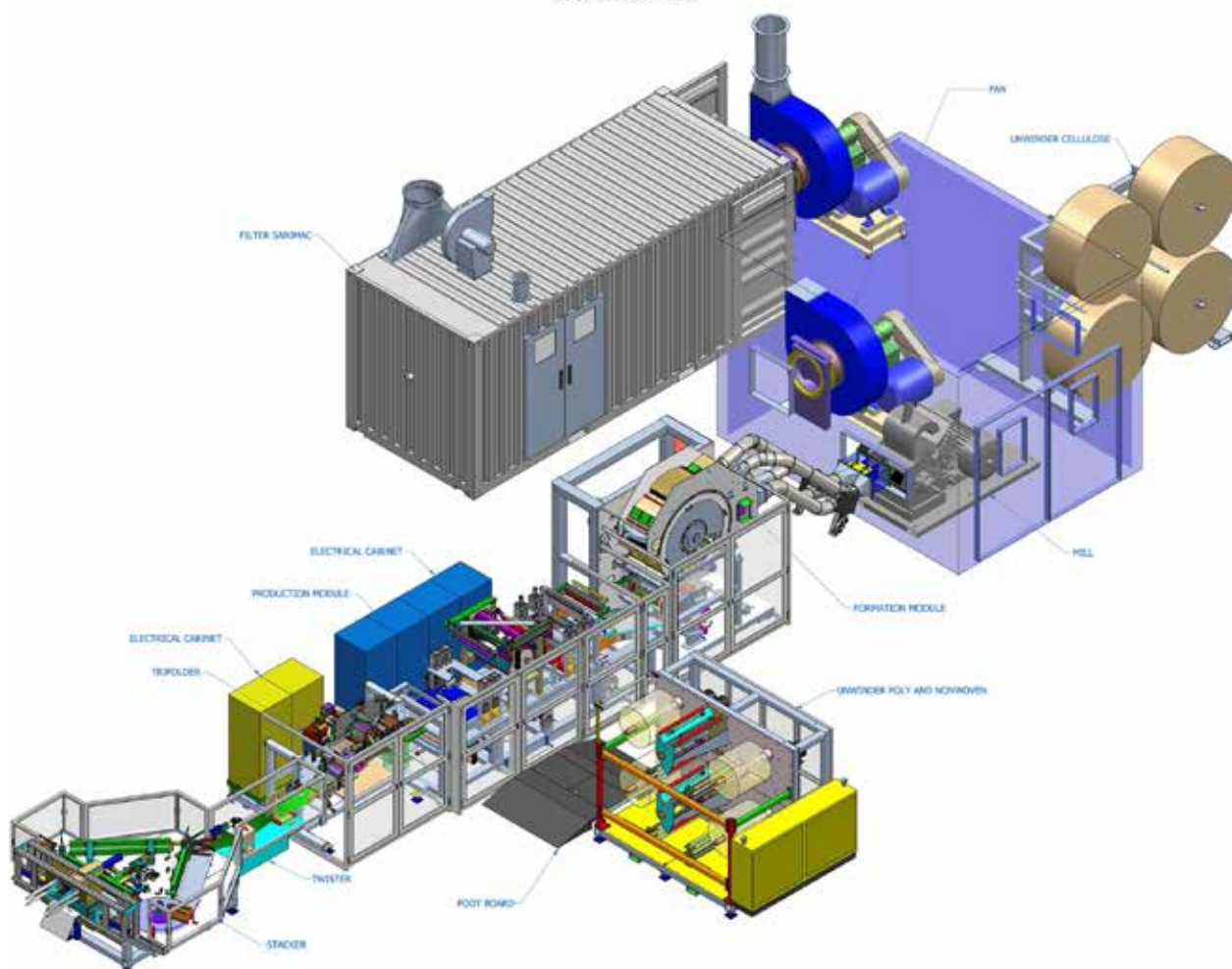
ISOMETRIC VIEW
